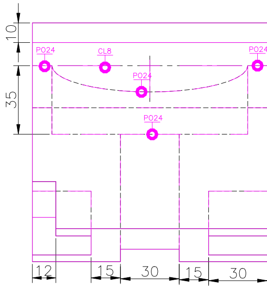
TOP SCALE 1/2
