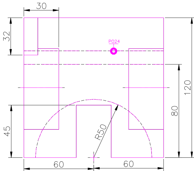
FRONT SCALE 1/2
