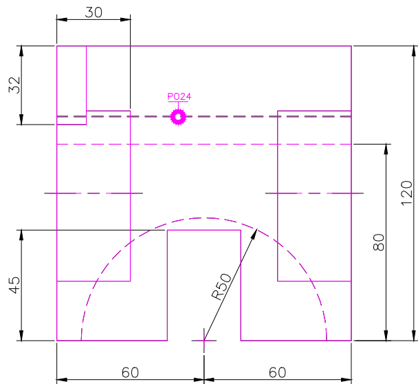
FRONT SCALE 1/2
