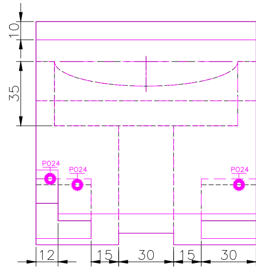
TOP SCALE 1/2
