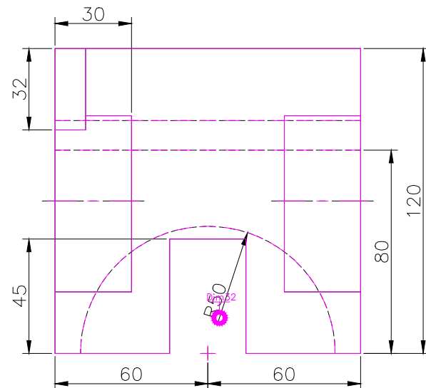
FRONT SCALE 1/2
