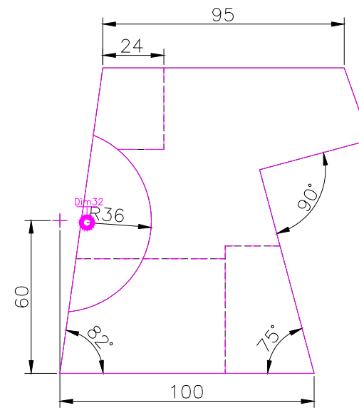
RIGHT SCALE 1/2
