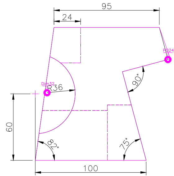
RIGHT SCALE 1/2
