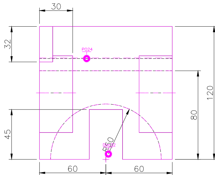
FRONT SCALE 1/2
