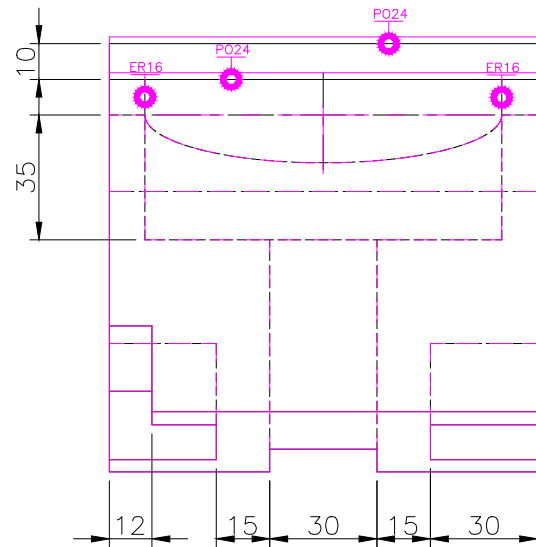
TOP SCALE 1/2
