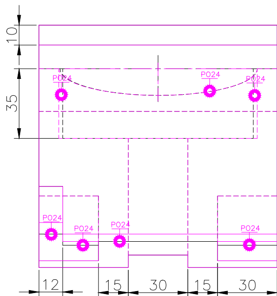
TOP SCALE 1/2
