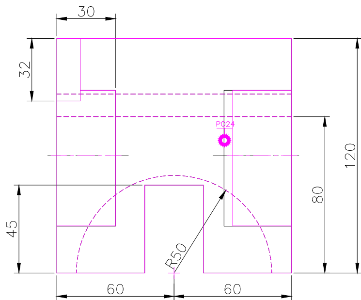
TOP SCALE 1/2
