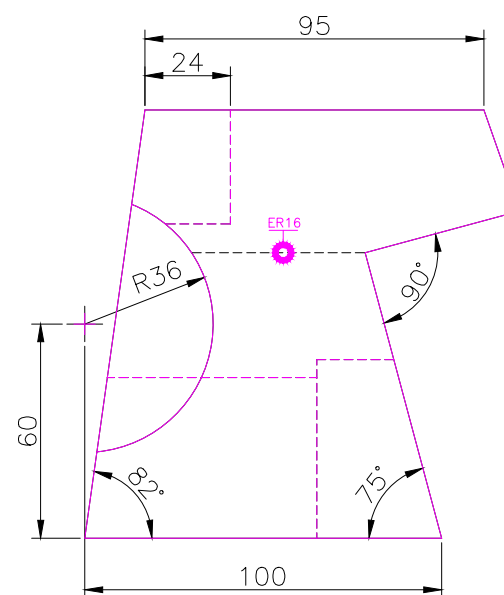
RIGHT SCALE 1/2
