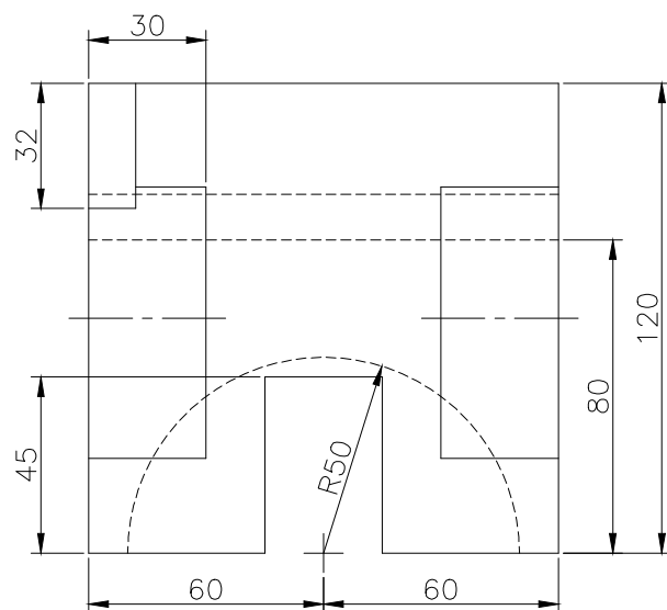
FRONT SCALE 1/2
