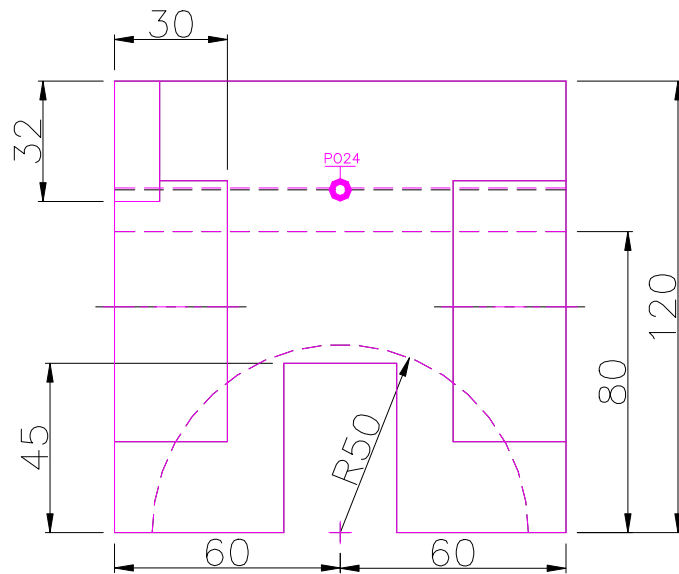
FRONT SCALE 1/2
