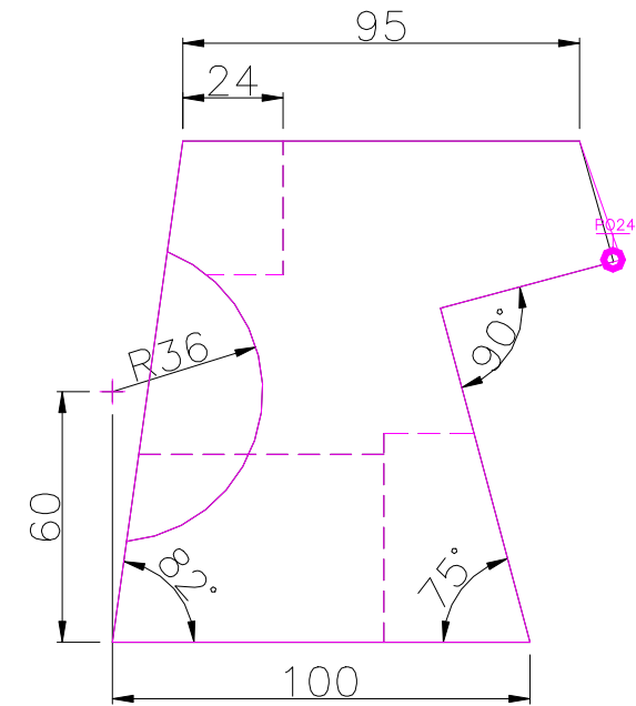
RIGHT SCALE 1/2
