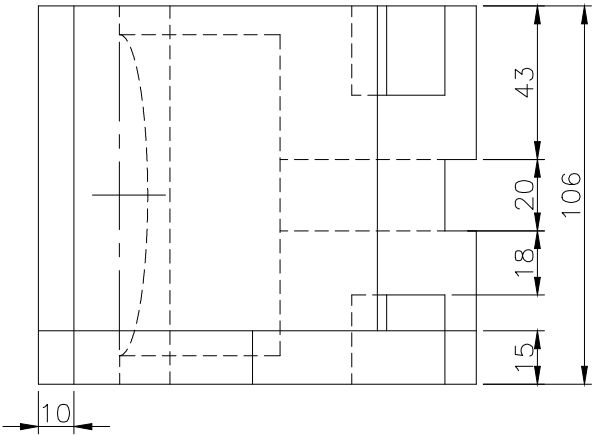
TOP SCALE 1/2
