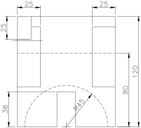
RIGHT SCALE 1/2
