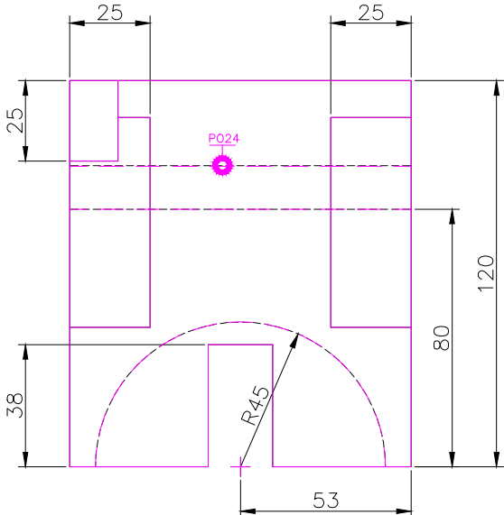
RIGHT SCALE 1/2
