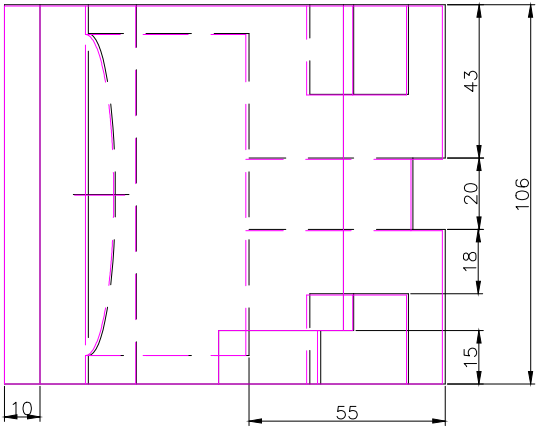
TOP SCALE 1/2
