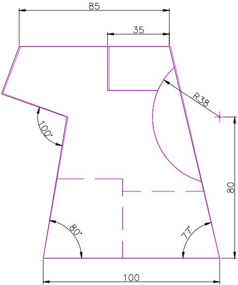
FRONT SCALE 1/2
