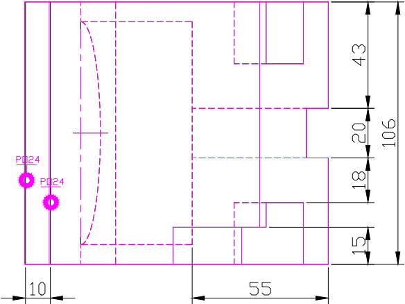
TOP SCALE 1/2
