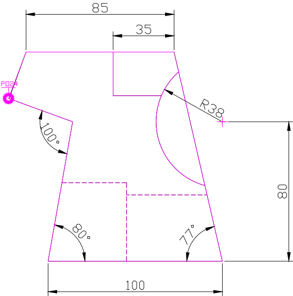
FRONT SCALE 1/2
