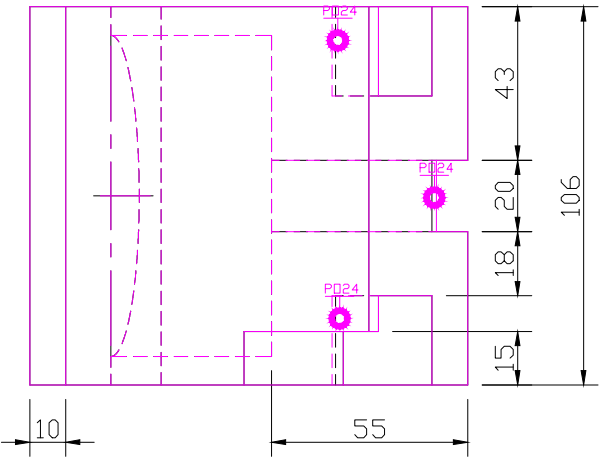
TOP SCALE 1/2
