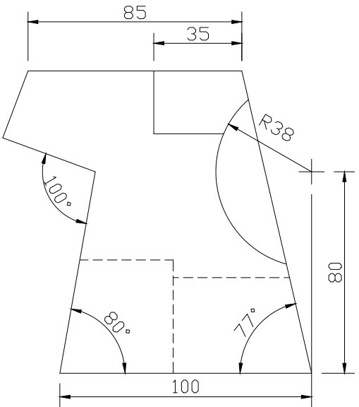
FRONT SCALE 1/2
