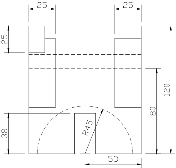
RIGHT SCALE 1/2
