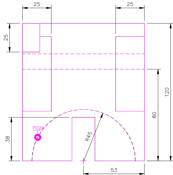
RIGHT SCALE 1/2
