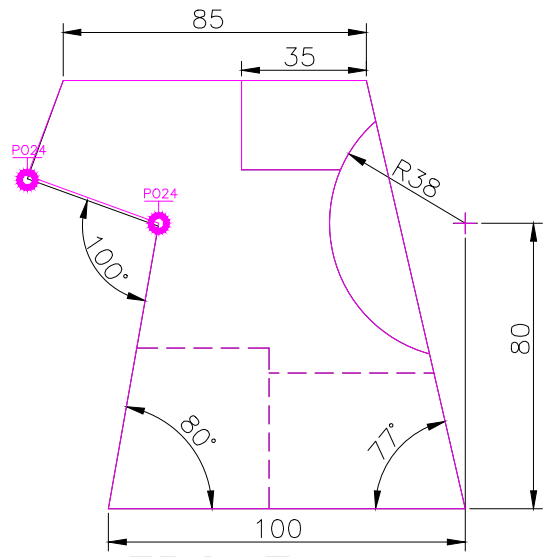
FRONT SCLAE 1/2
