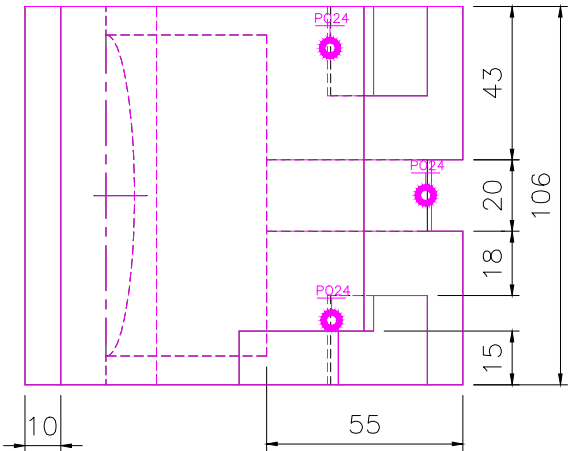
TOP SCALE 1/2
