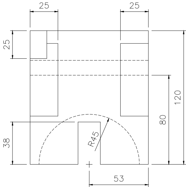
RIGHT SCALE 1/2
