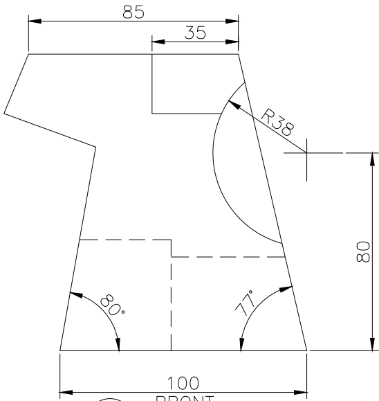
FRONT SCALE 1/2
