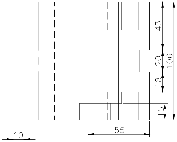
TOP SCALE 1/2
