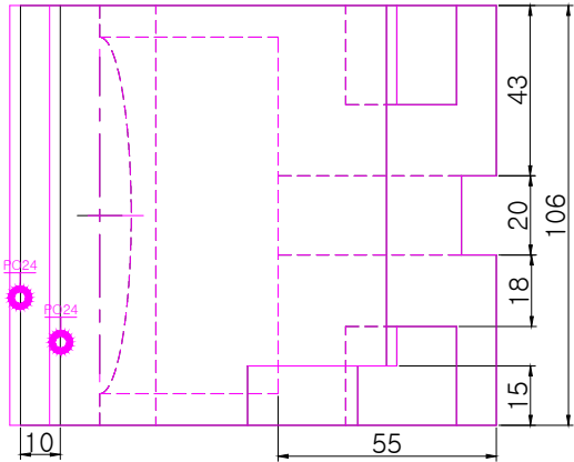
TOP SCALE 1/2
