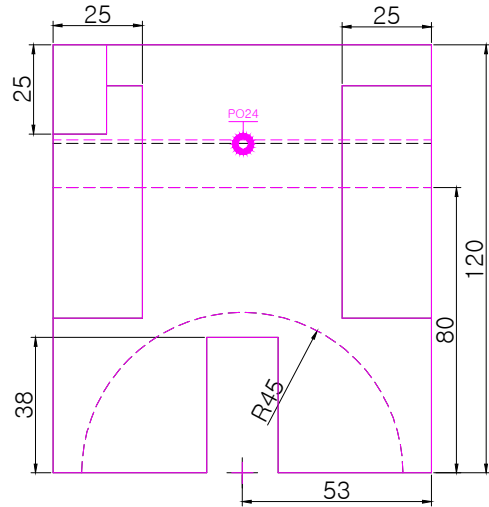
RIGHT SCALE 1/2
