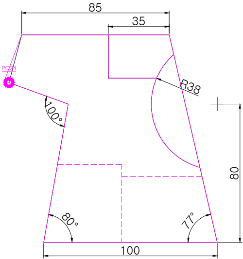
FRONT SCALE 1/2
