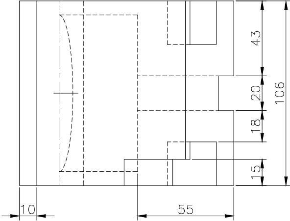
TOP SCALE 1/2
