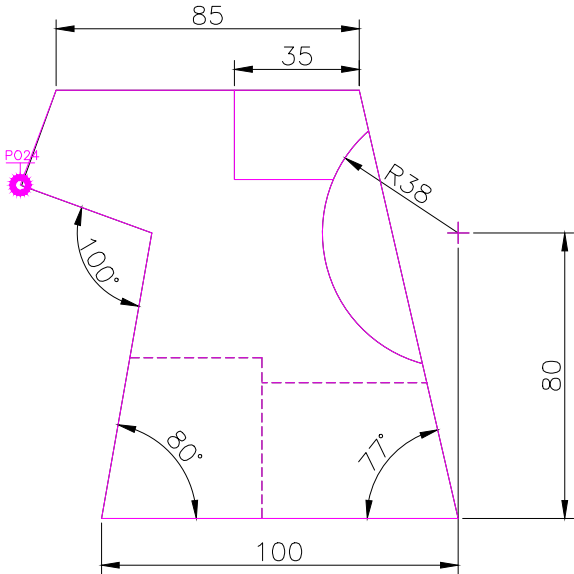
FRONT SCALE 1/2
