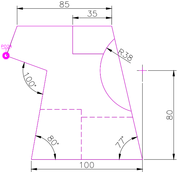
FRONT SCALE 1/2
