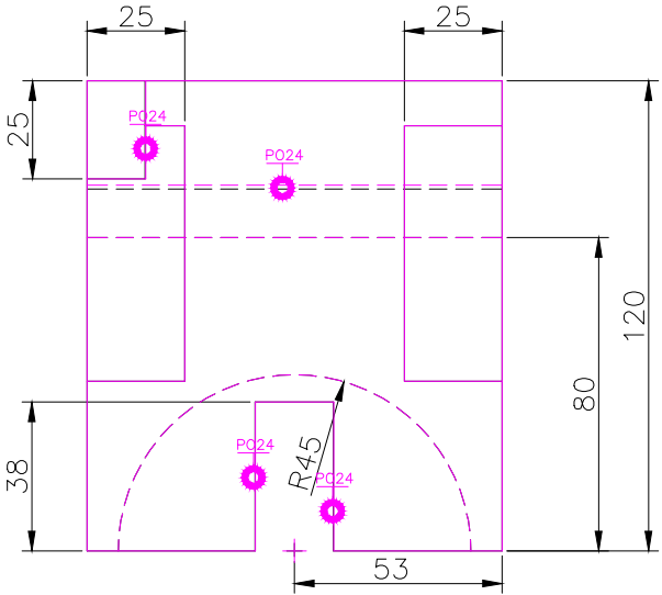
RIGHT SCALE 1/2
