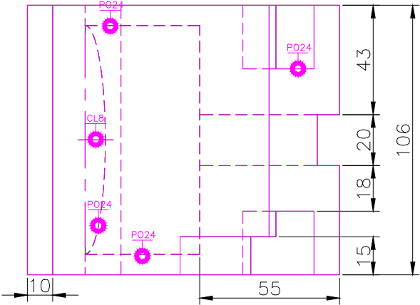
TOP SCALE 1/2
