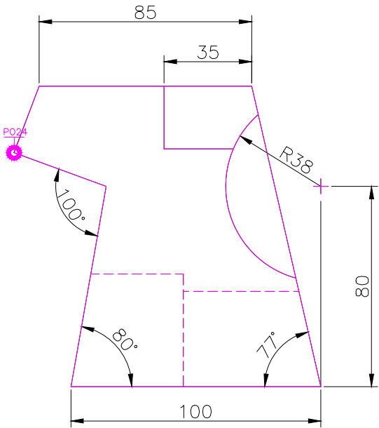
FRONT SCALE 1/2
