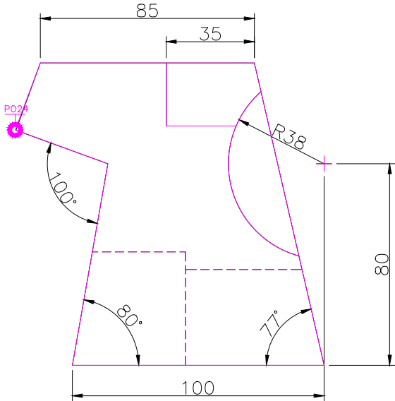
FRONT SCALE 1/2
