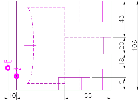
TOP SCALE 1/2
