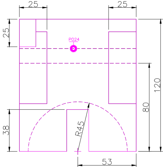
RIGHT SCALE 1/2
