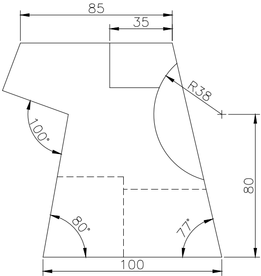
FRONT SCALE 1/2
