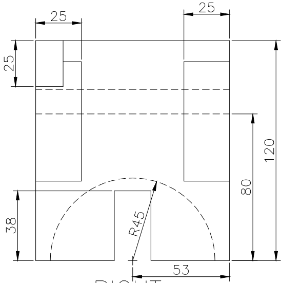
RIGHT SCALE 1/2
