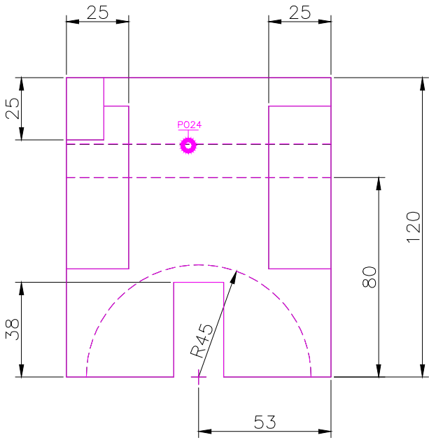
RIGHT SCALE 1/2
