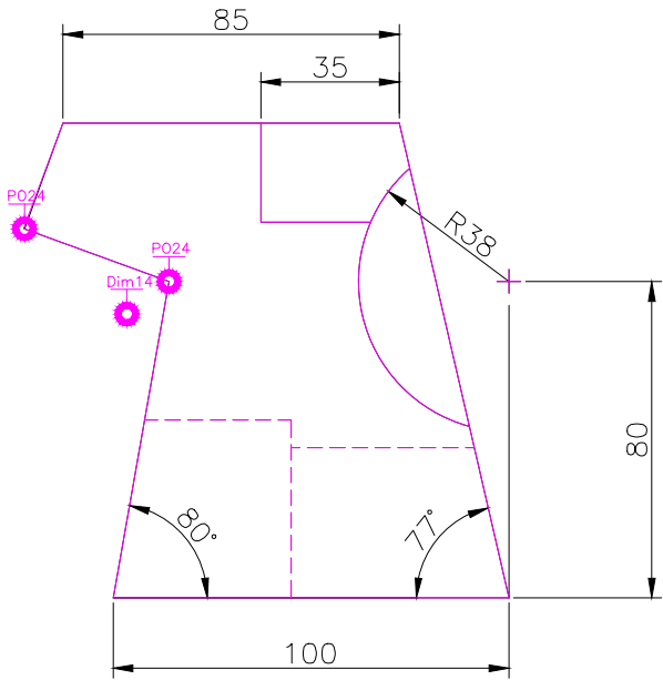
FRONT SCALE 1/2
