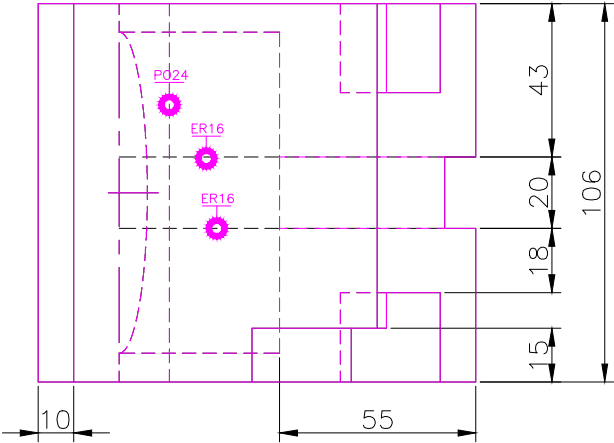
TOP SCALE 1/2
