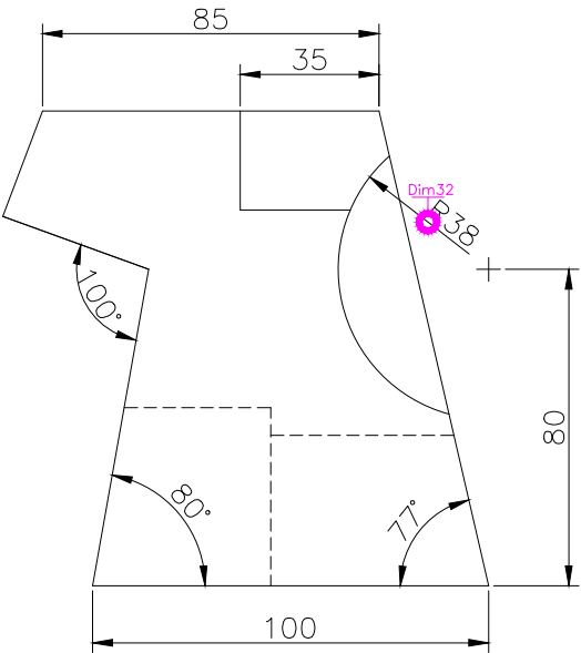
FRONT SCALE 1/2
