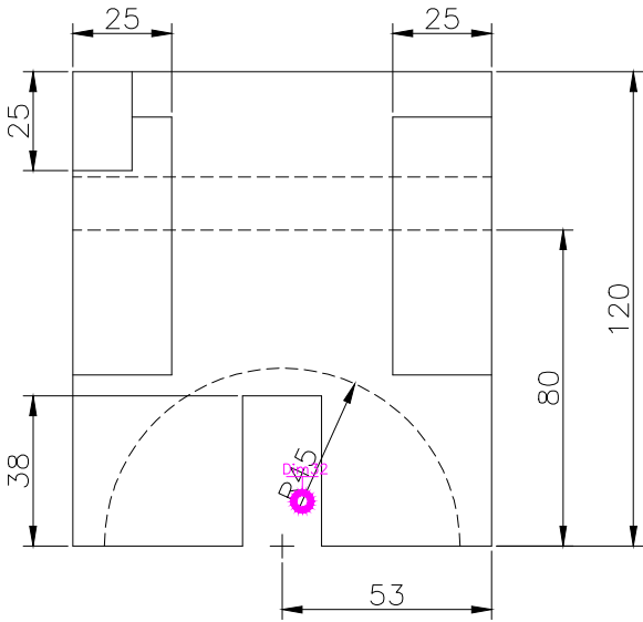
RIGHT SCALE 1/2
