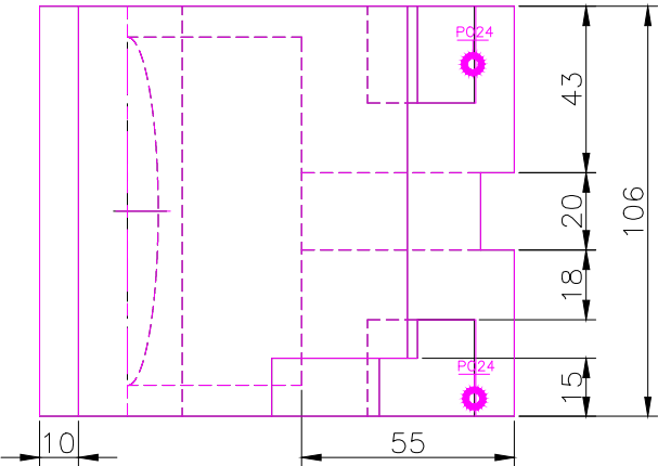
TOP SCALE 1/2
