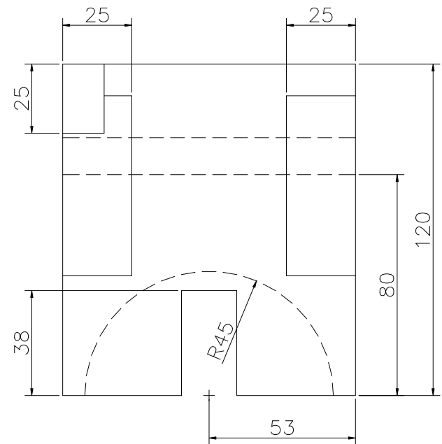
RIGHT SCALE 1/2
