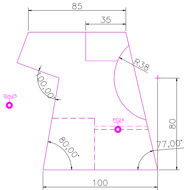
FRONT SCALE 1/2
