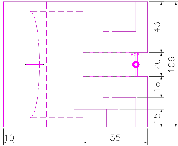
TOP SCALE 1/2
