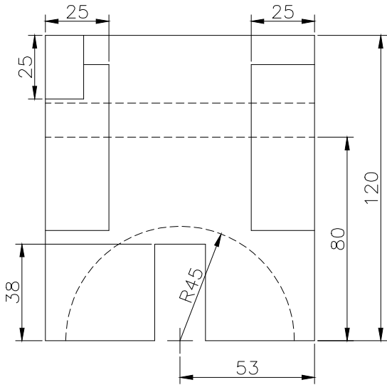
RIGHT SCALE 1/2
