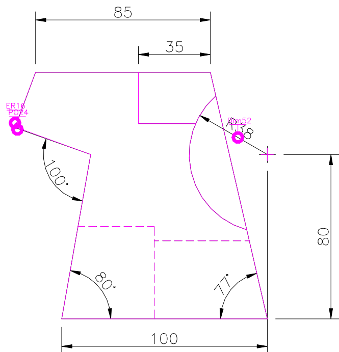
FRONT SCALE 1/2
