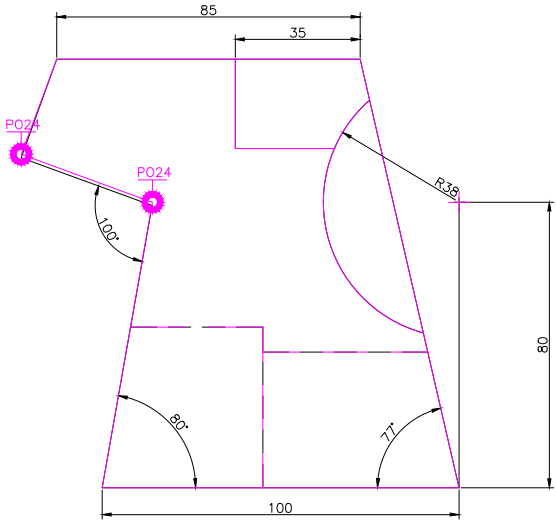
FRONT SCALE 1/2
