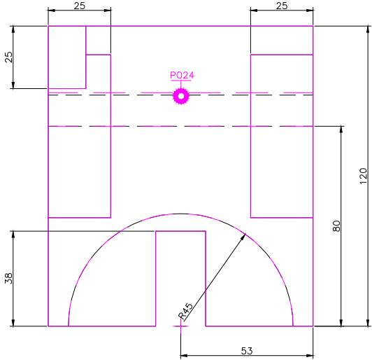
RIGHT SCALE 1/2
