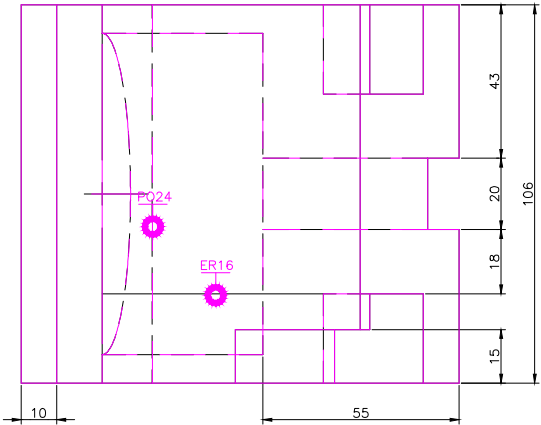
TOP SCALE 1/2
