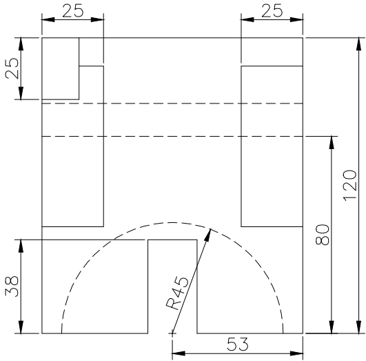
RIGHT SCALE 1/2
