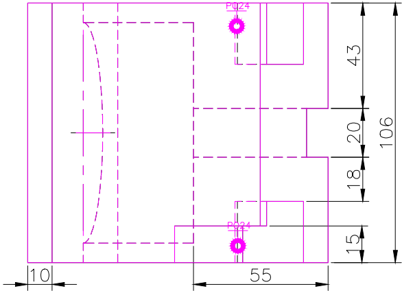
TOP SCALE 1/2
