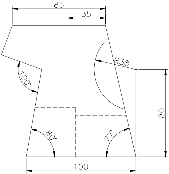
FRONT SCALE 1/2
