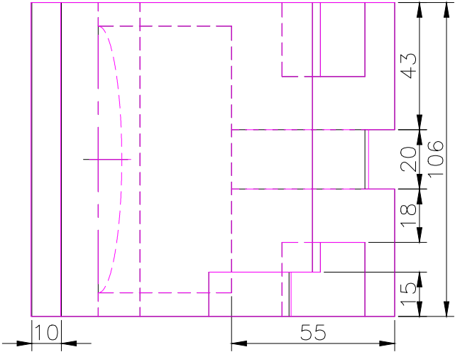
TOP SCALE 1/2
