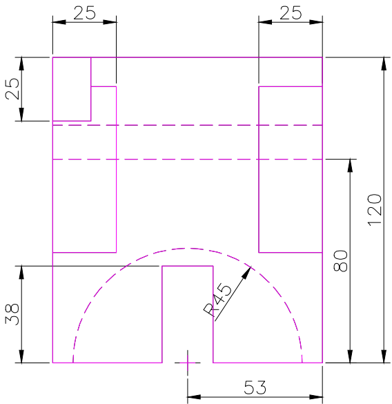
RIGHT SCALE 1/2
