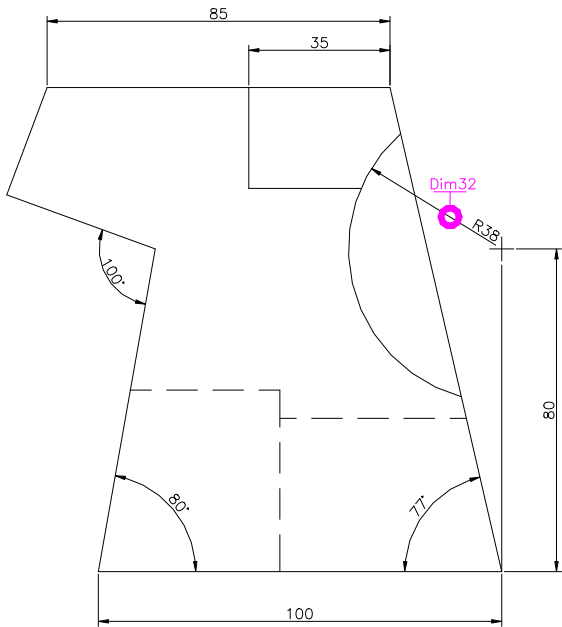
FRONT SCALE 1/2
