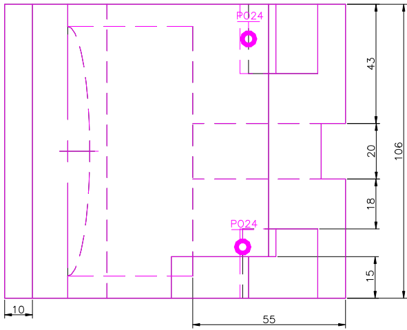
TOP SCALE 1/2
