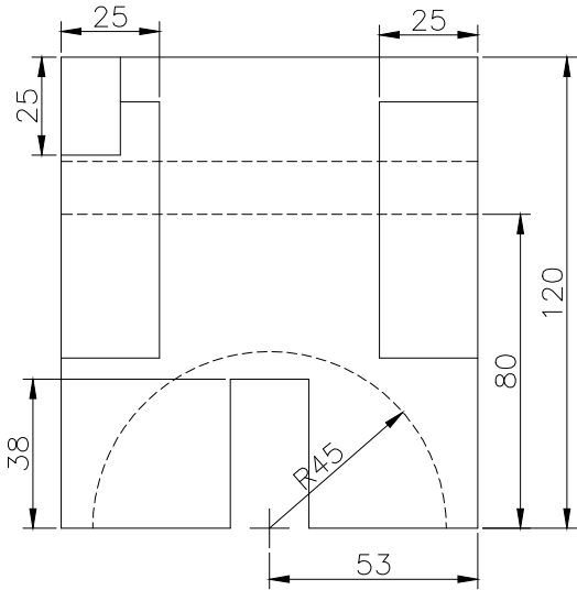
RIGHT SCALE 1/2
