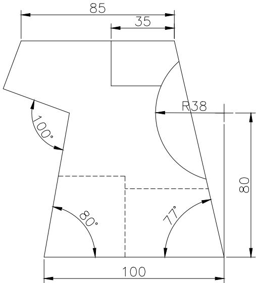
FRONT SCALE 1/2
