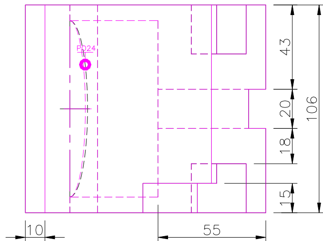
TOP SCALE 1/2
