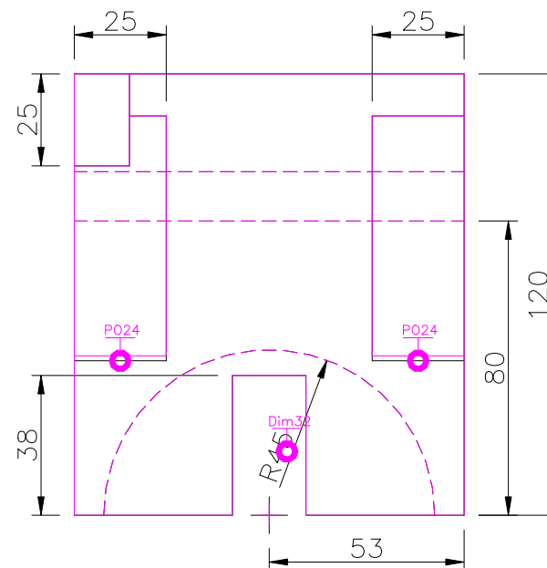
RIGHT SCALE 1/2
