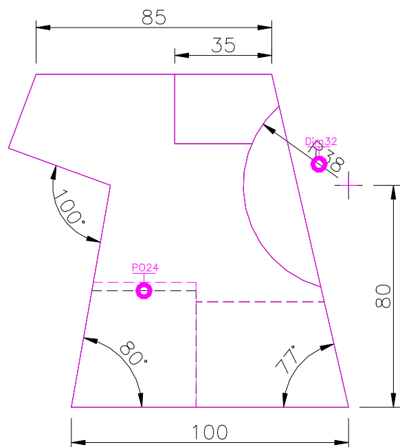
FRONT SCALE 1/2
