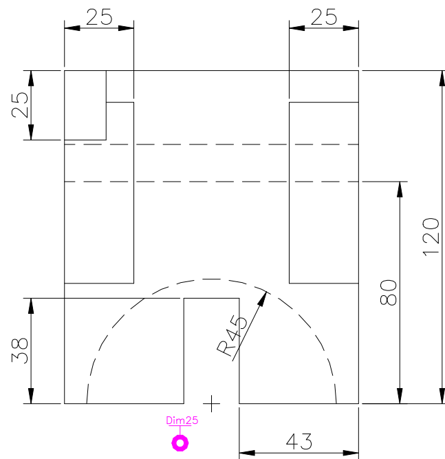
RIGHT SCALE 1/2
