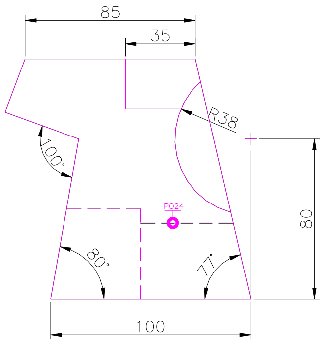
FRONT SCALE 1/2
