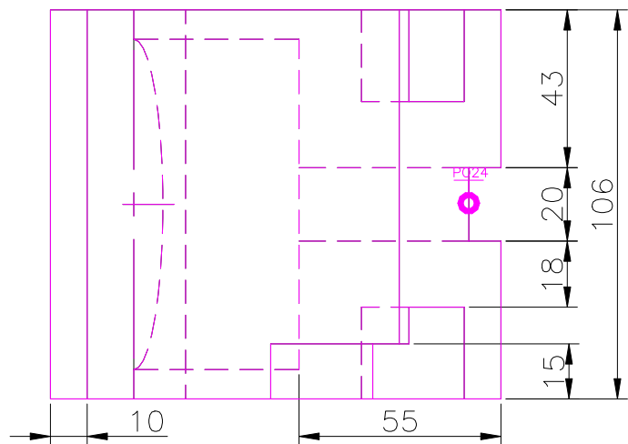
TOP SCALE 1/2
