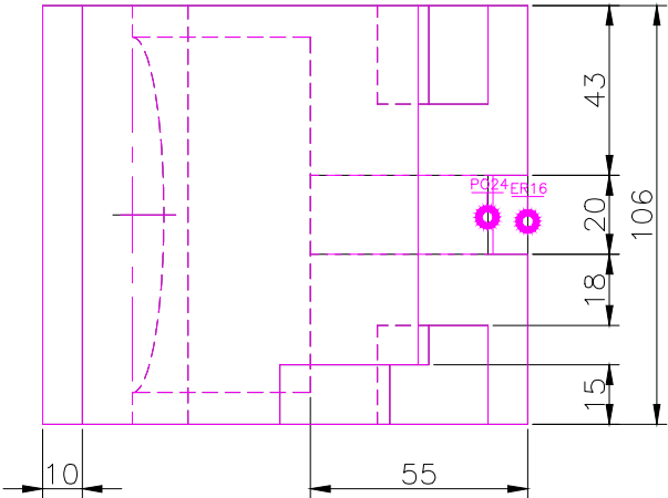
TOP SCALE 1/2
