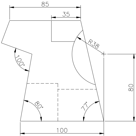
FRONT SCALE 1/2
