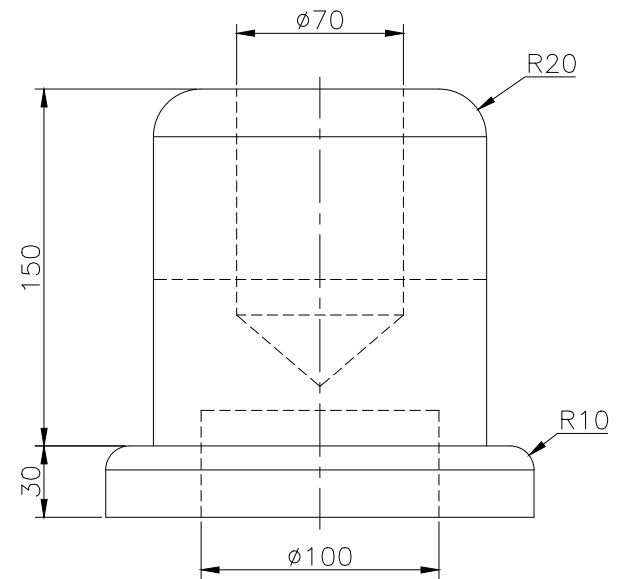
RIGHT SCALE 1/3
