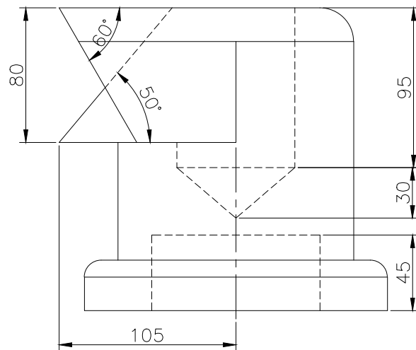
FRONT SCALE 1/3
