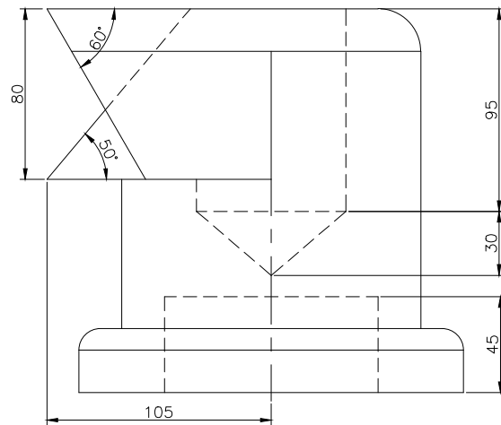
FRONT SCALE 1/3
