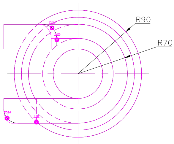
TOP SCALE 1/3
