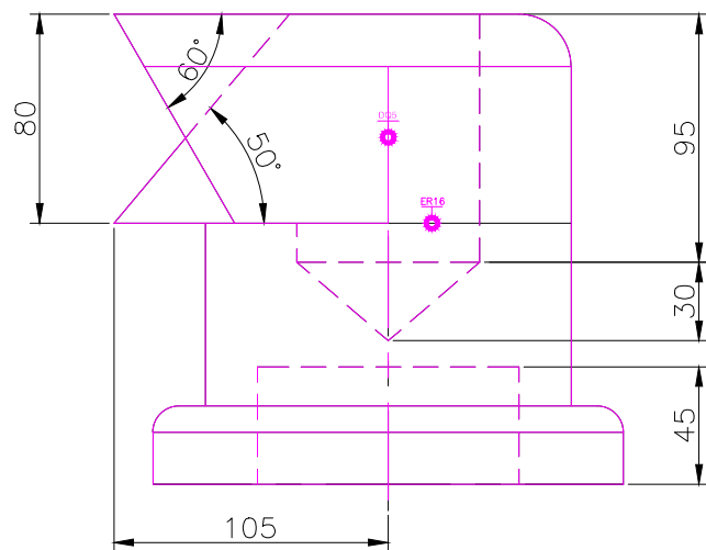
FRONT SCALE 1/3
