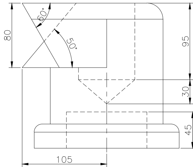
FRONT scale 1/3
