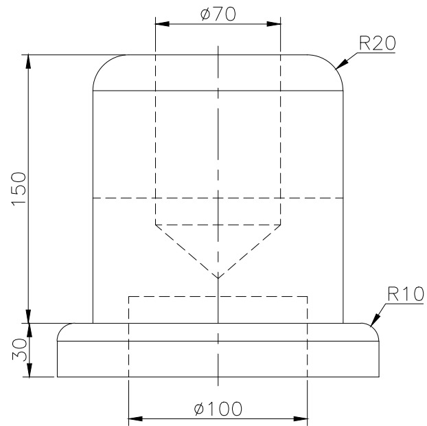
RIGHT scale 1/3
