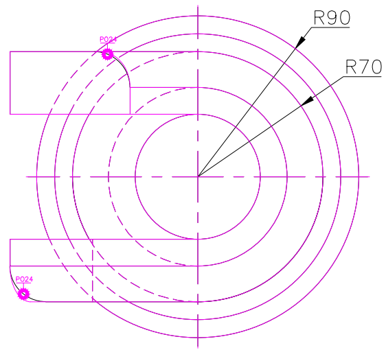
TOP scale 1/3
