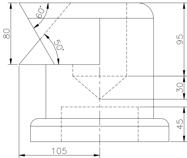
FRONT SCALE 1/3
