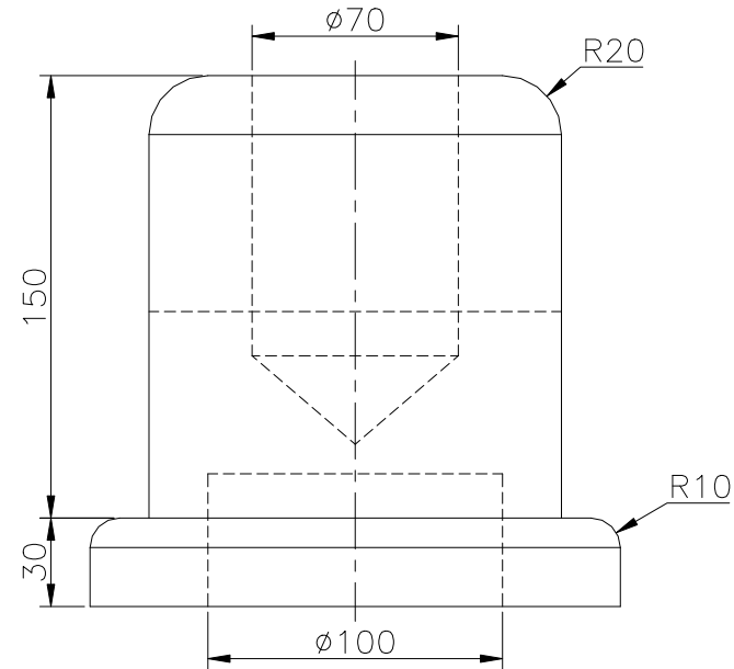
RIGHT SCALE 1/3
