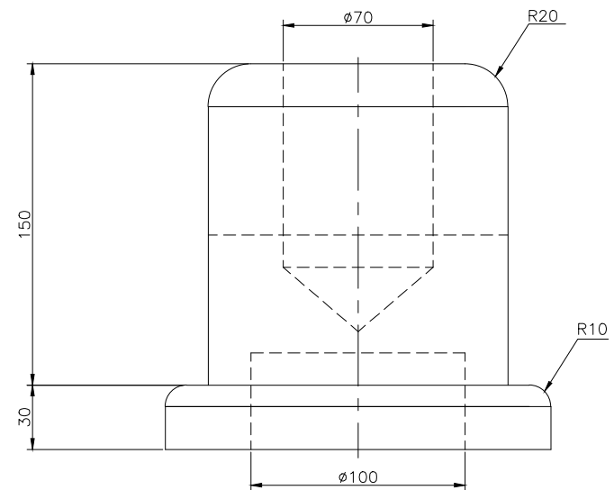
RIGHT SCALE 1/3
