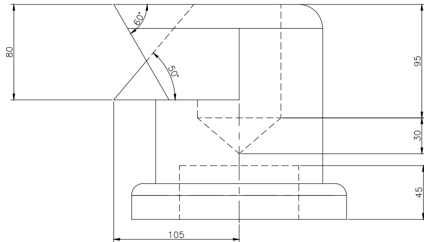
FRONT SCALE 1/3
