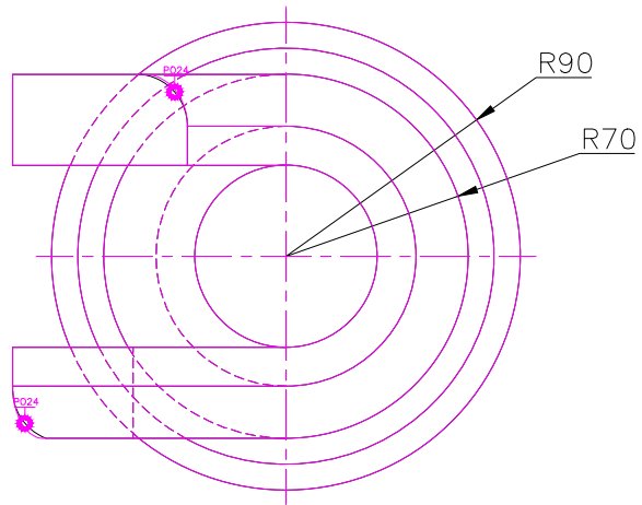
TOP SCALE 1/3
