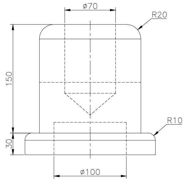
RIGHT SCALE 1/3
