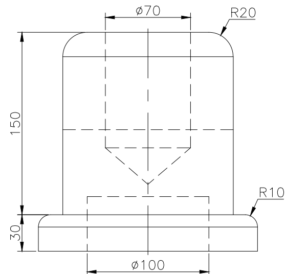
RIGHT SCALE 1/3
