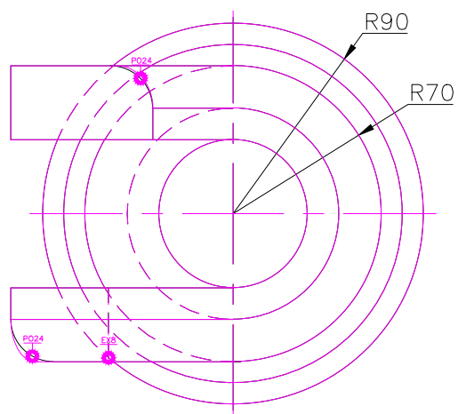
TOP SCALE 1/3
