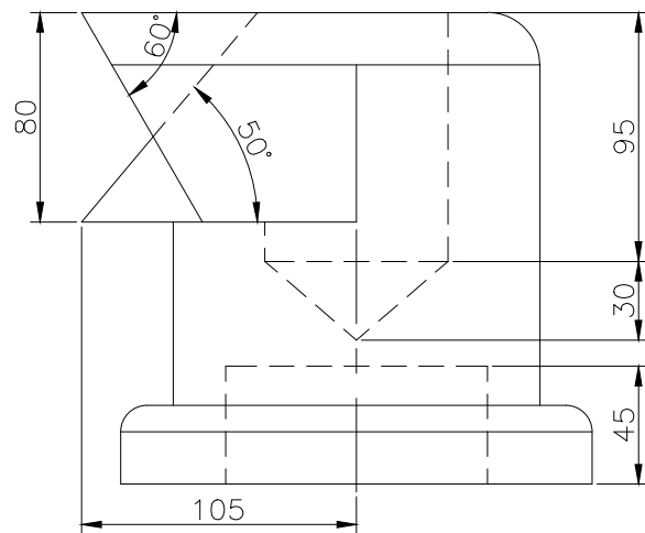
FRONT SCALE 1/3
