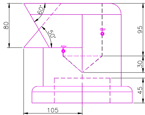
FRONT SCALE 1/3
