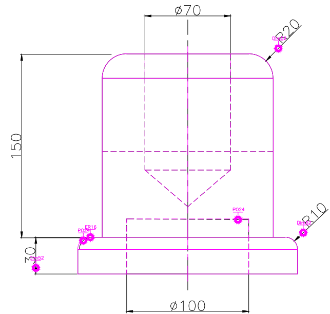
RIGHT SCALE 1/3
