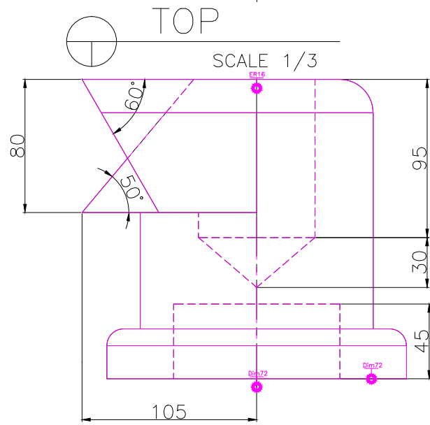
FRONT SCALE 1/3
