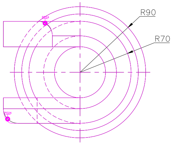
TOP SCALE 1/3
