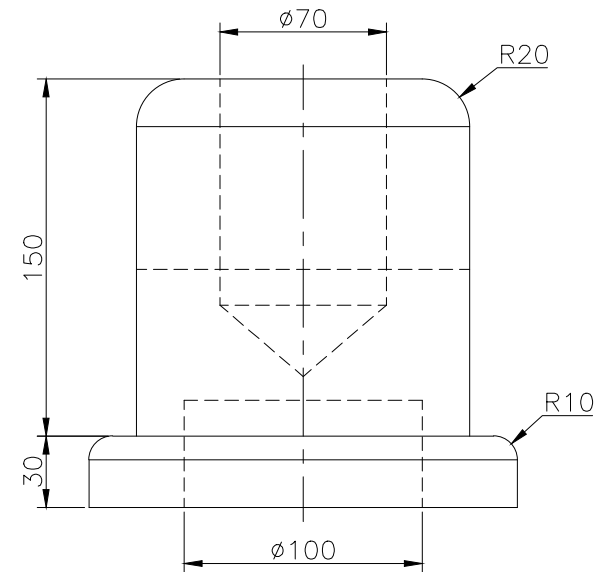
RIGHT SCALE 1/3
