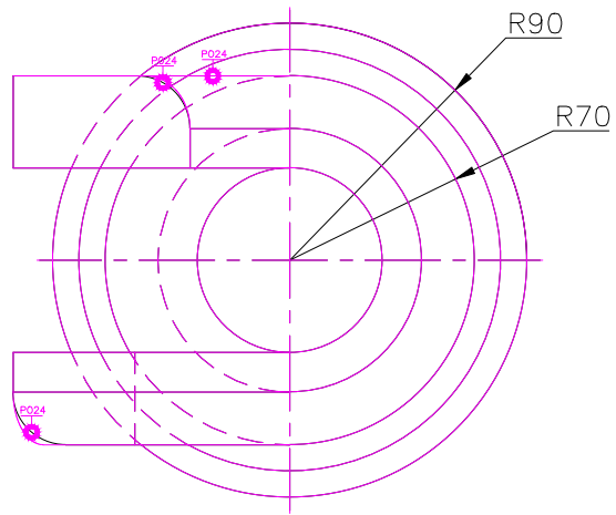
TOP SCALE 1/3
