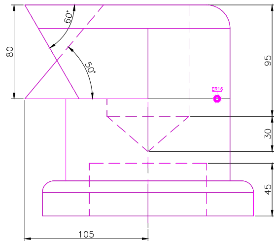
FRONT SCALE 1/3
