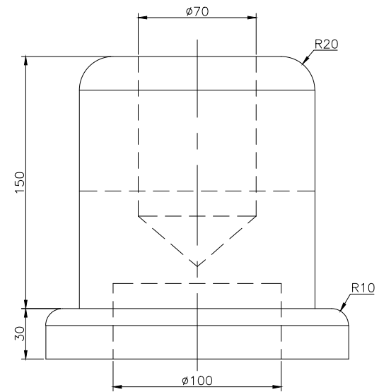
RIGHT SCALE 1/3
