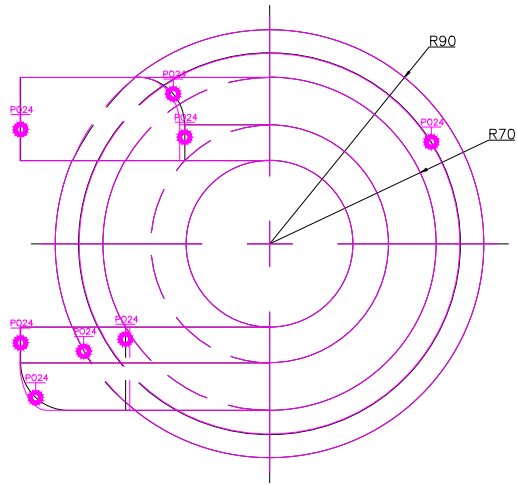
TOP SCALE 1/3
