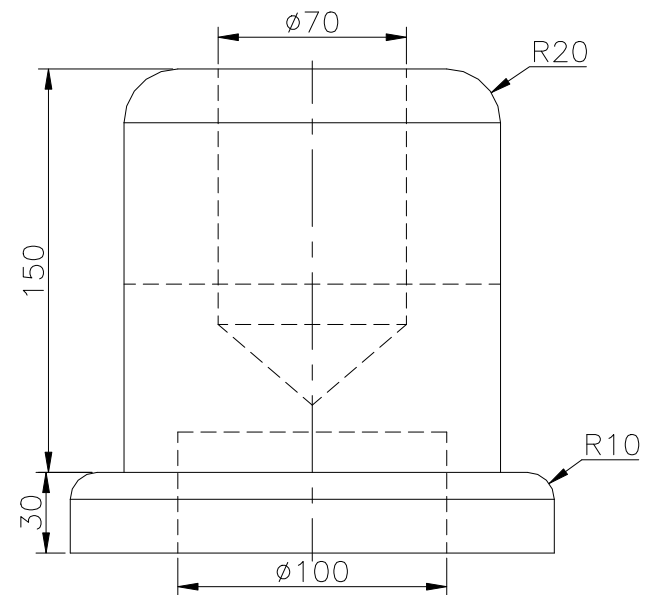
RIGHT SCALE 1/3
