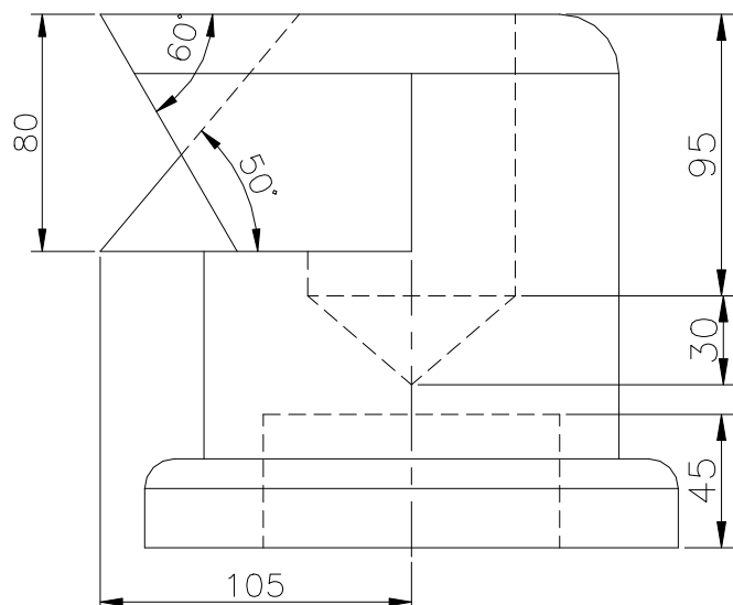
FRONT SCALE 1/3
